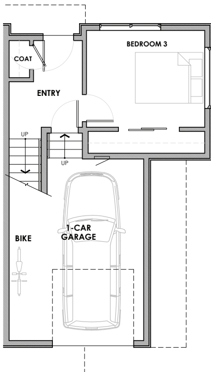
TH4 - Level 1
