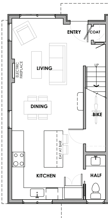
TH3 - Level 1
