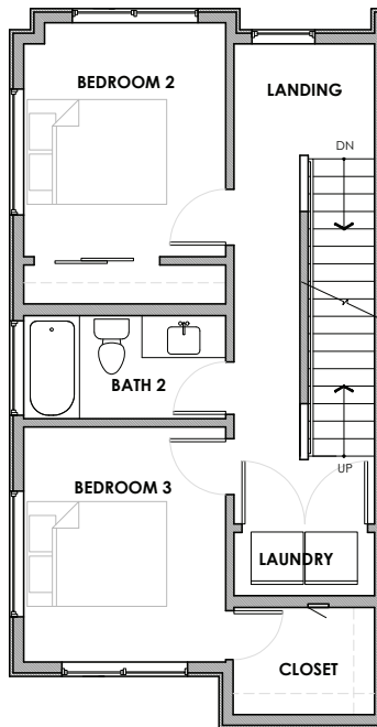
TH3 - Level 2
